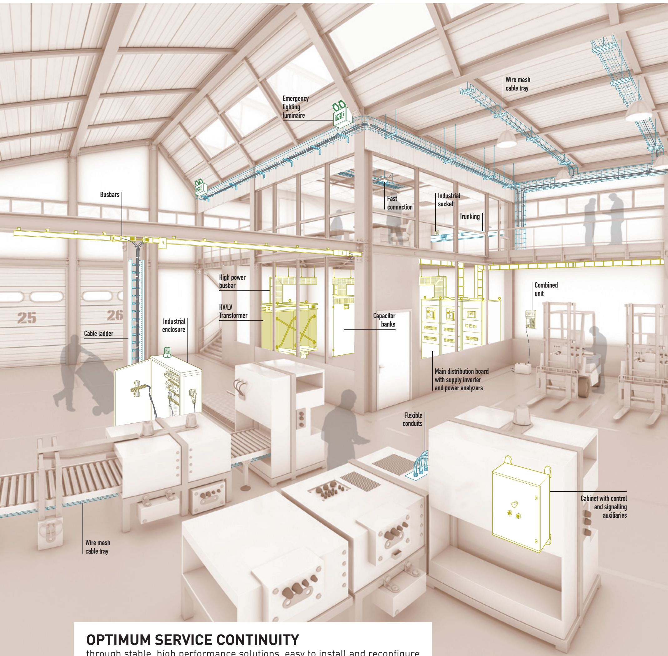
Swifts cable ladder: main distribution infrastructure
